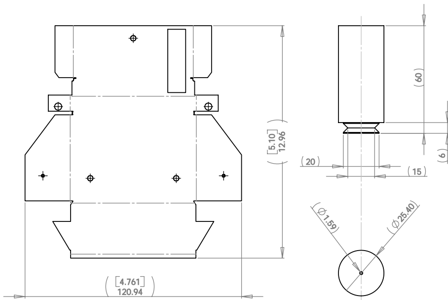
ButtFighter FRAME and CYLINDER
