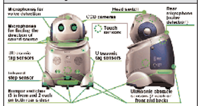
Figure 10. PaPeRo sensors.
